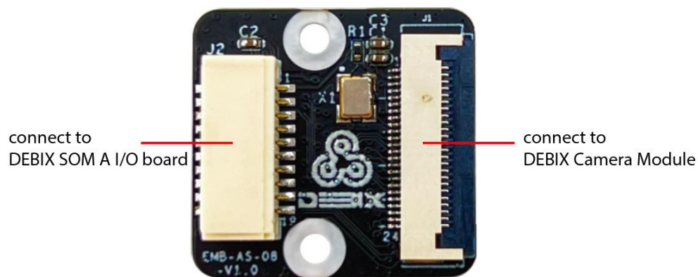
Figure 7 Camera Adapter Board for DEBIX SOM A I/O Board
